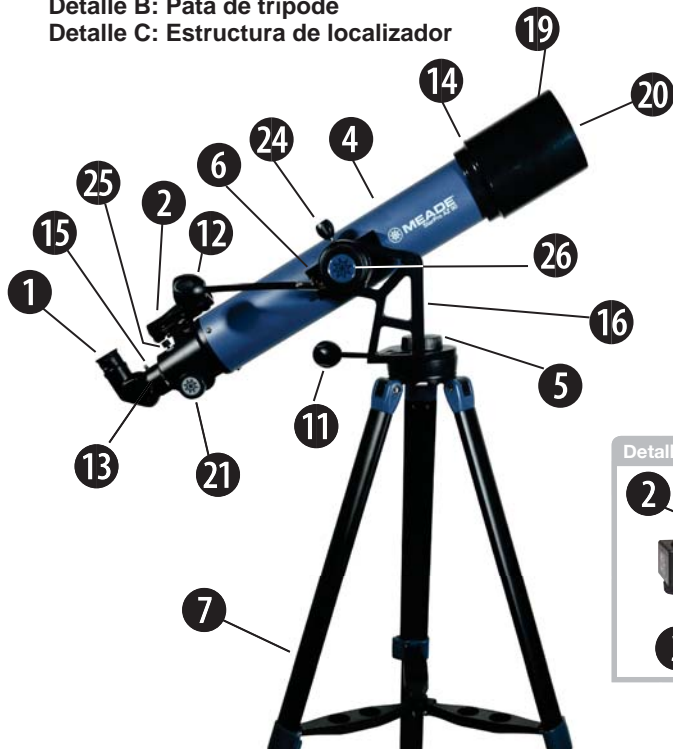
Figura 1: Telescopio refractor altazimut Meade StarPro™ AZ
